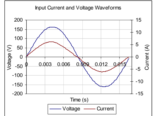
Input AC Current Waveform (ITHD = 11.96%, 50% Load)
