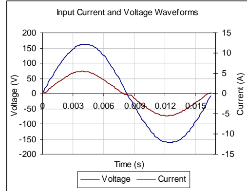
Input AC Current Waveform (ITHD = 14.64%, 50% Load)
