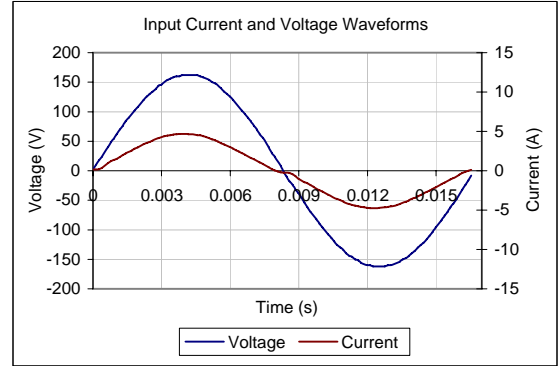
Input AC Current Waveform (ITHD = 13.1%, 50% Load)
