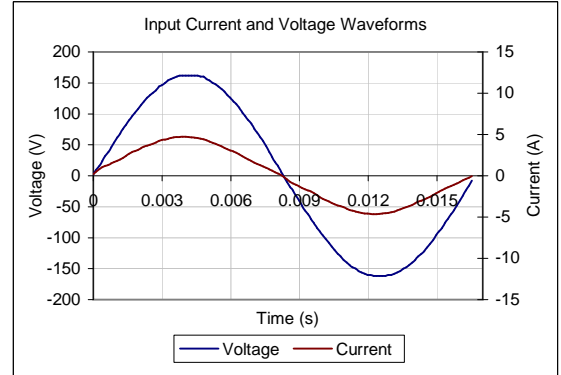
Input AC Current Waveform (ITHD = 6.31%, 50% Load)
