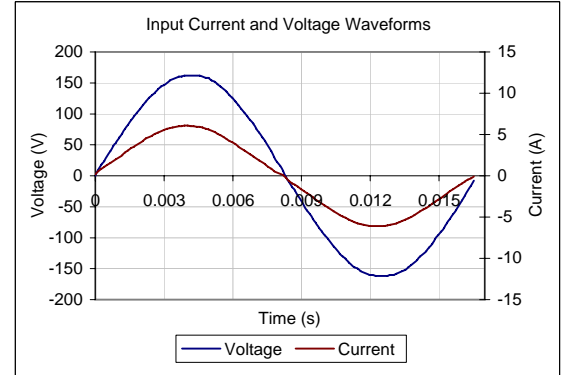
Input AC Current Waveform (ITHD = 5%, 50% Load)
